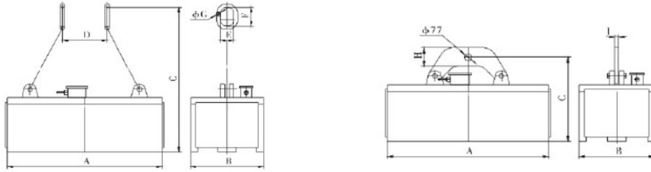
M22吊鋼坯常溫型技術參數 Technical data for normal temperature type
